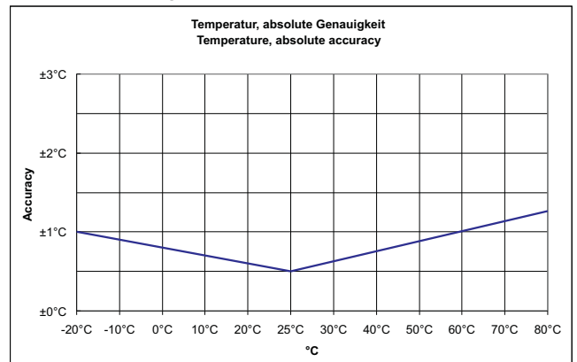
Temperatur FTA 54 VV / FTA 54 AA Temperature FTA 54 VV / FTA 54 AA
