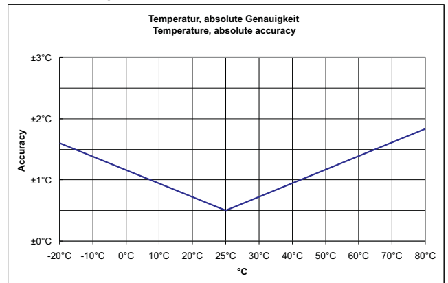
Temperatur LC-FTA 54 VV / LC-FTA 54 AA Temperature LC-FTA 54 VV / LC-FTA 54 AA
