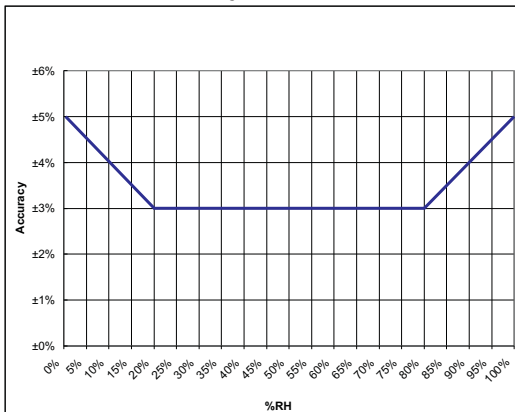
rel. Feuchte LC-FA 54 / LC-FTA 54 rel. Humidity LC-FA 54 / LC-FTA 54
