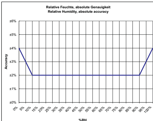
rel. Feuchte FA 54 / FTA 54 rel. Humidity FA 54 / FTA 54
