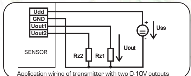
Application wiring of transmitter with two 0-10V outputs
