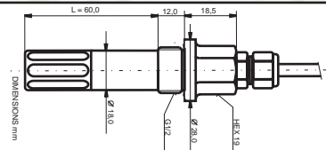
TO211P transmitter T+RH, dewpoint metal probe for compressed air up to 20 bars
