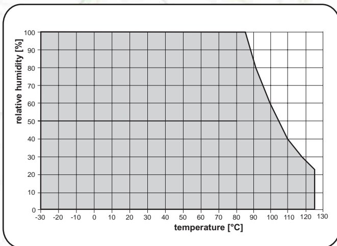
TO211P transmitter T+RH, dewpoint metal probe for compressed air up to 20 bars
