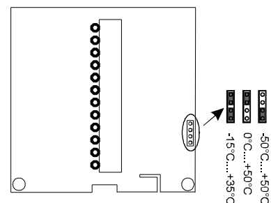
Messbereichseinstellung Measuring range adjustment
