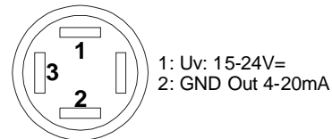
4-20mA Type
